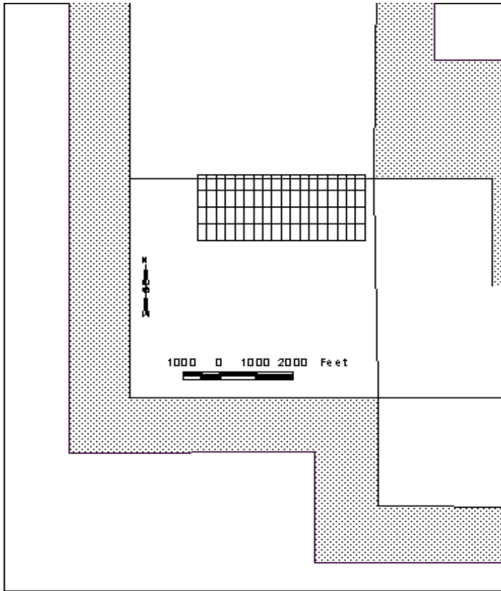
Figure 8. Example placement grid within the HARS (used for the KVK Phase II, Contract I dredging project). The area of the grid is 1,000,000 yd 2 . The estimated 1,293,000 yd 3 of dredged material from the project provided an average coverage of approximately 4 ft (~1.2m) within the grid.
