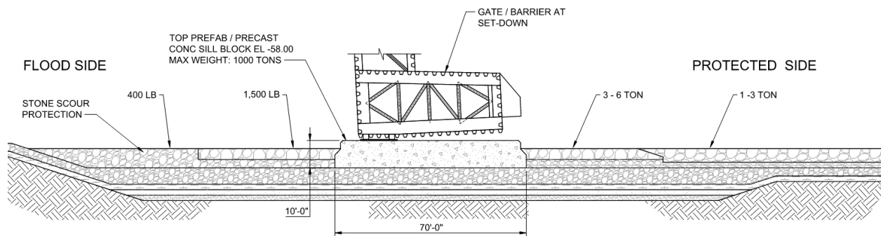
Figure 3-5 Floating Sector Gate Sill
