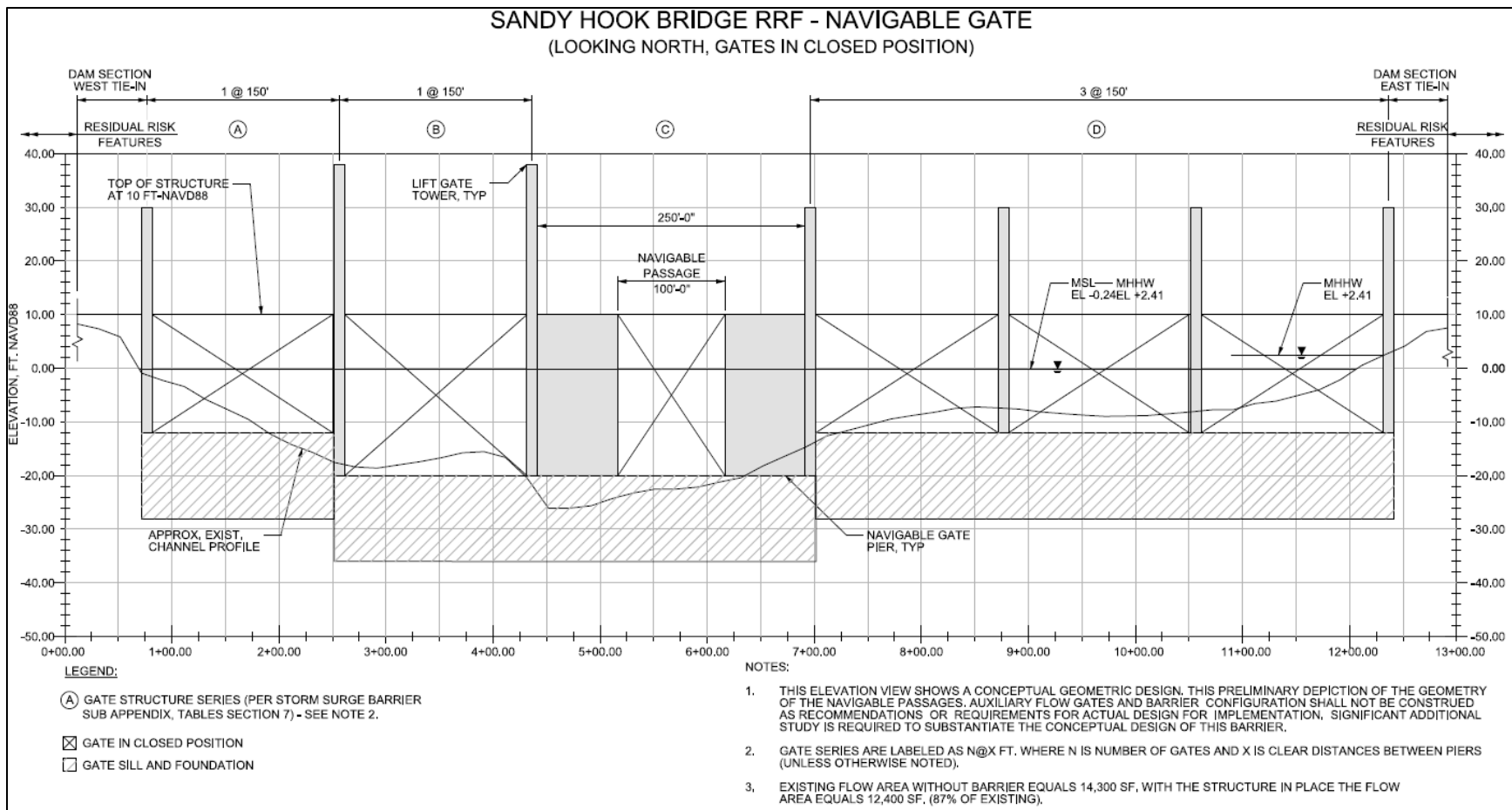
Figure 7-5 Conceptual Geometry of Gates of the Sandy Hook Bridge RRF Navigable Gate
