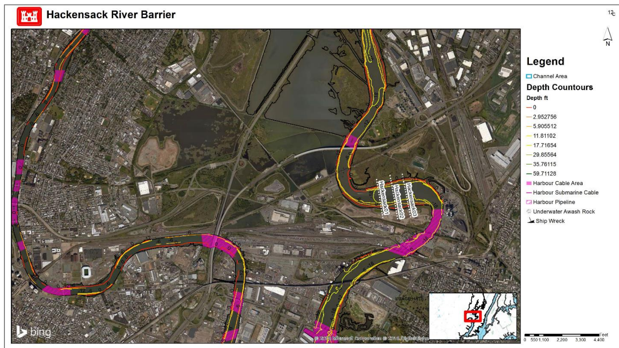
Figure 5-1 Area of Interest for the Hackensack Storm Surge Barrier Which Spans the Hackensack River in New Jersey
