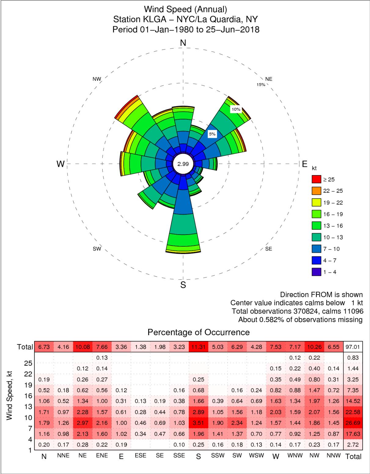
Figure 2-5 Percentage of Occurrence for Wind Speed in knots for La Guardia Airport (Station KLGA) for a 38-year period
