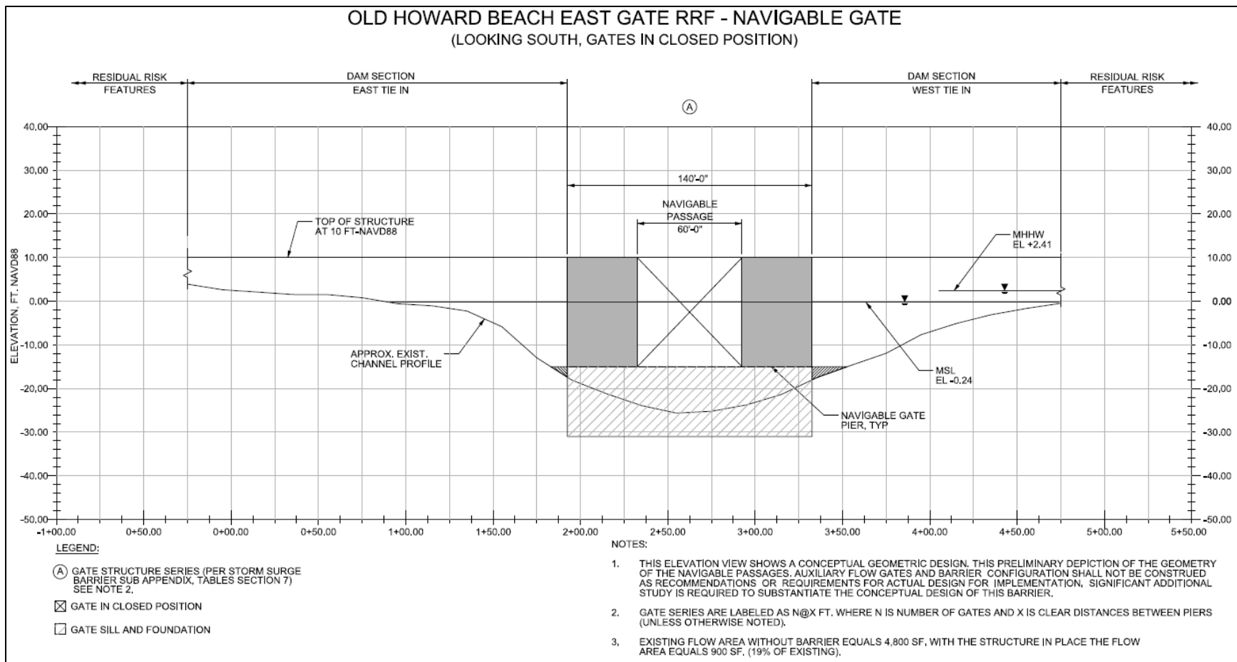
Figure 7-9 Conceptual Geometry of Gates of the Old Howard Beach East Gate RRF Navigable Gate
