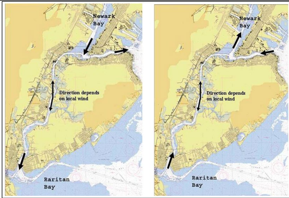
Figure 19: Current direction influenced by wind under typical conditions. (Chant 2006)
