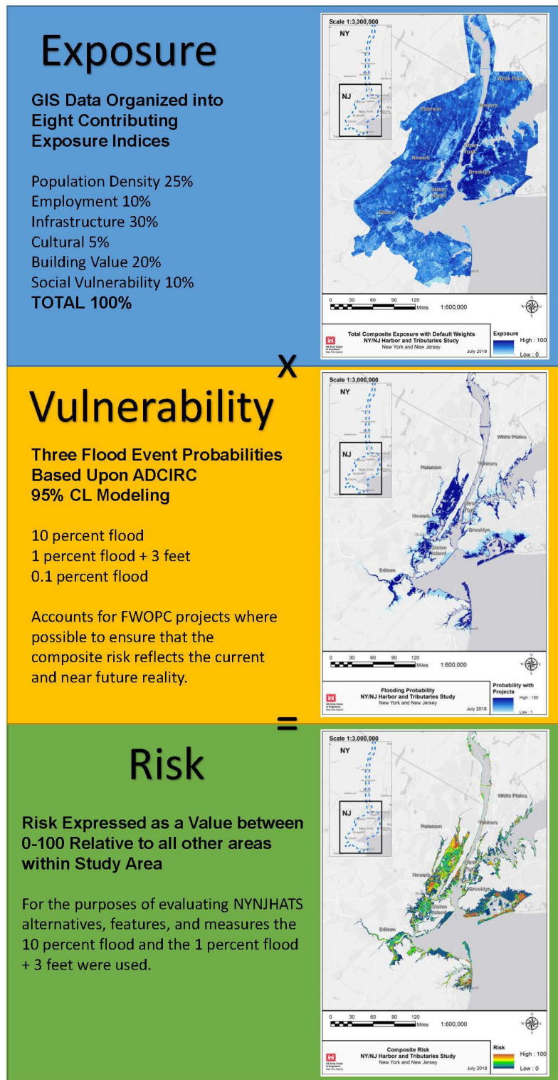
Figure 3. Risk Calculation
