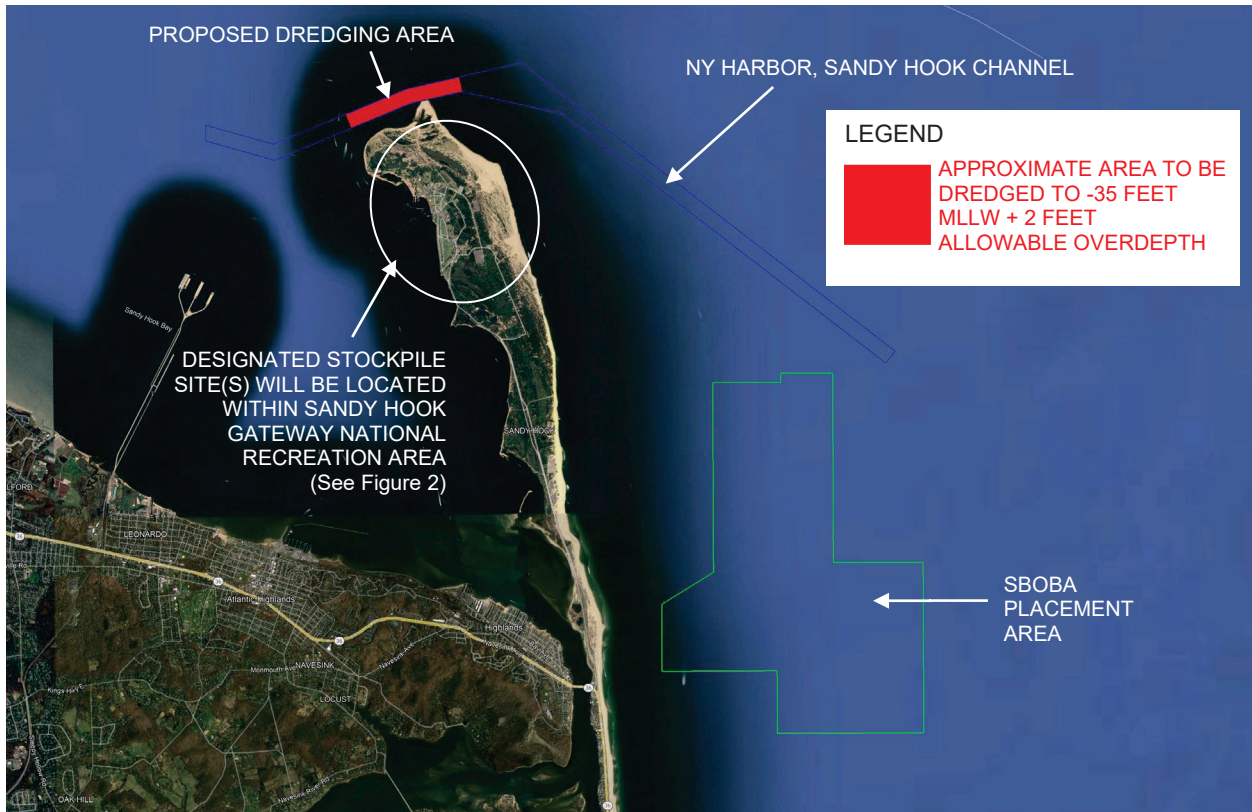
Figure 1: Dredging and Placement Location Map (Not to scale)
