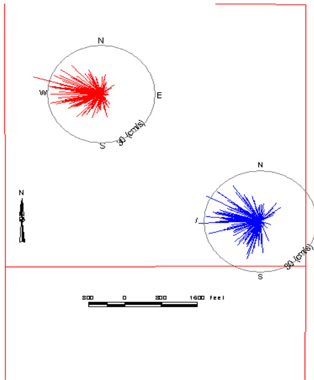
Figure 11. Current meter data from ARESS pods deployed in HARS PRA#1 from 15 –29 October 1998. Data are from sensors 15cm above the bottom
