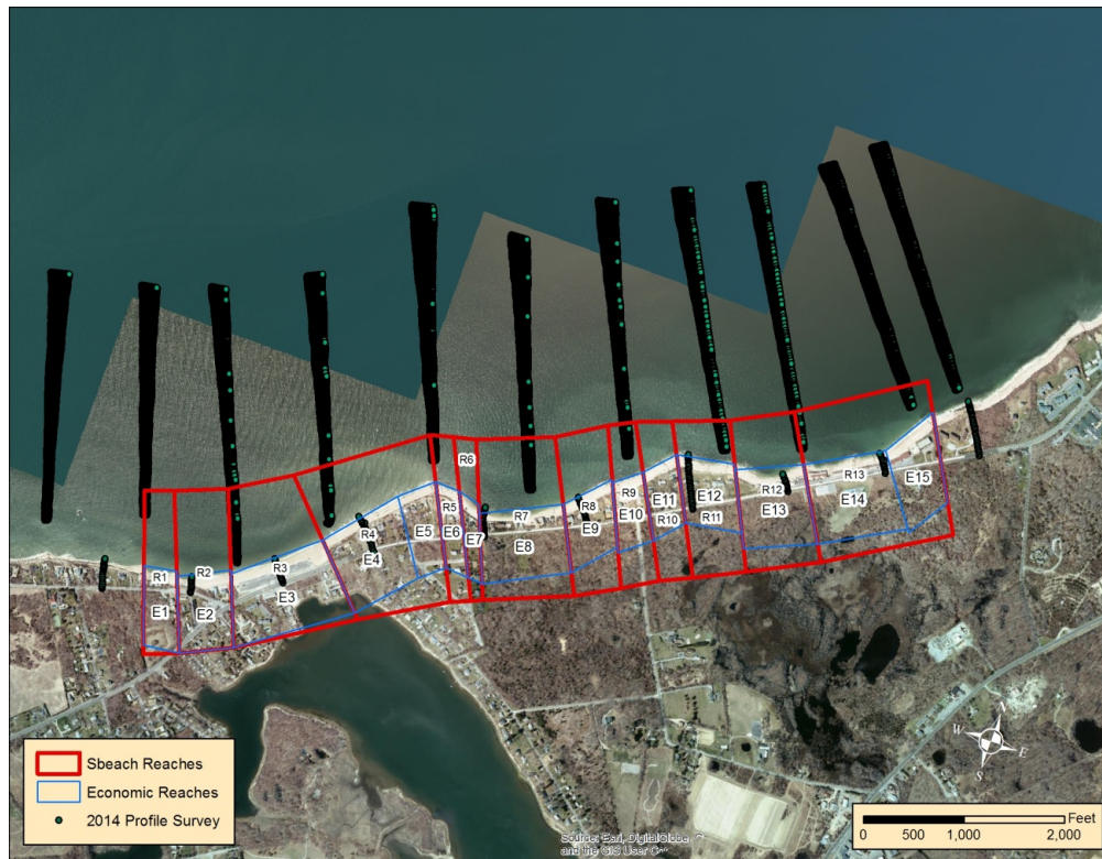
Figure 17: Profile Survey Transects
