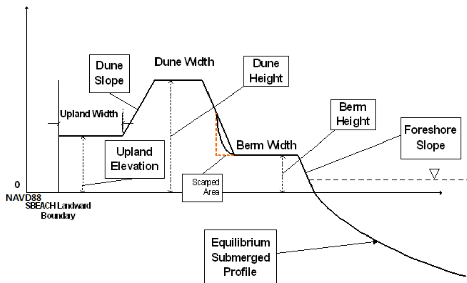
Figure 15: Beach-fx idealized beach profile.
