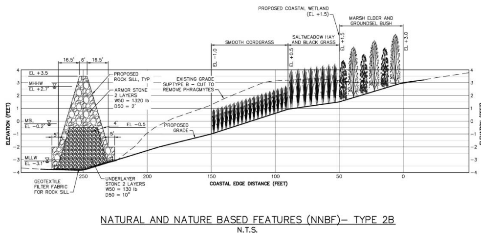
Figure 4-19: NNBF Feature Type 1A, 1B, 2A and 2B Cross-Sections
