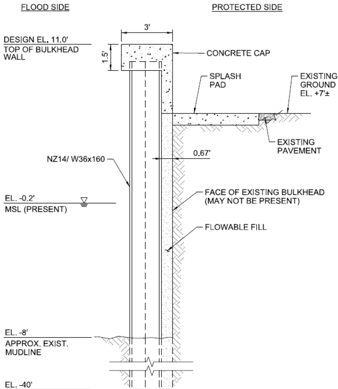
Figure 4-10: Deep Bulkhead Cross-Section
