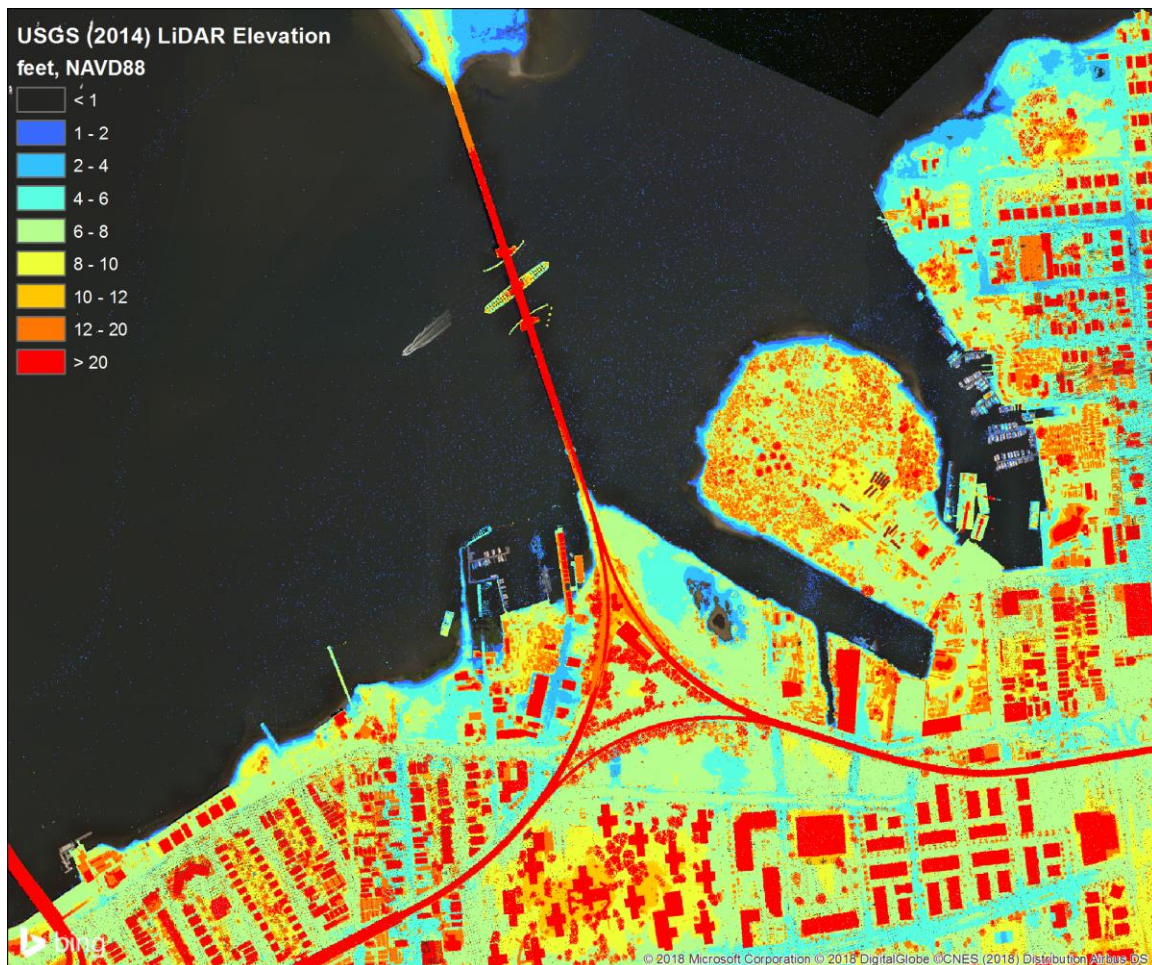
Figure 2-2: Map showing LiDAR Elevations extracted for Hammels vicinity, Rockaway
