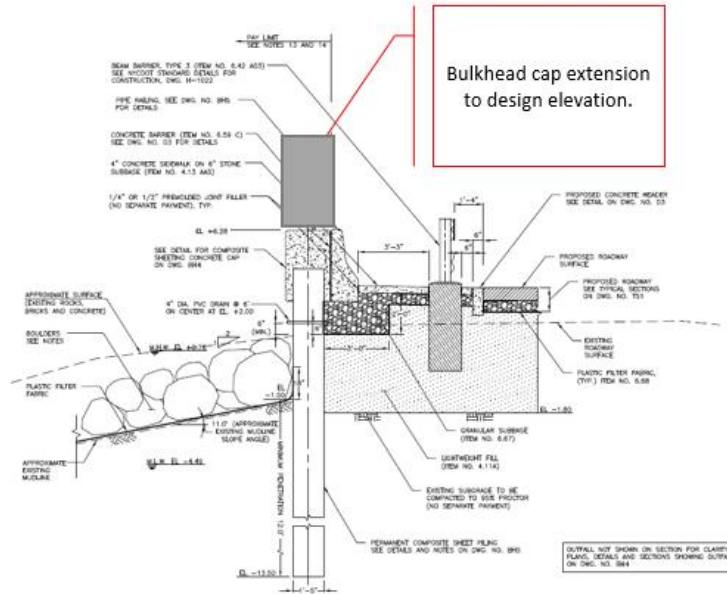
Figure 4-12: Street End Bulkhead Cross-Section (typical section taken from DDC Project ID-HWQ1182A for illustrative purposes only)
