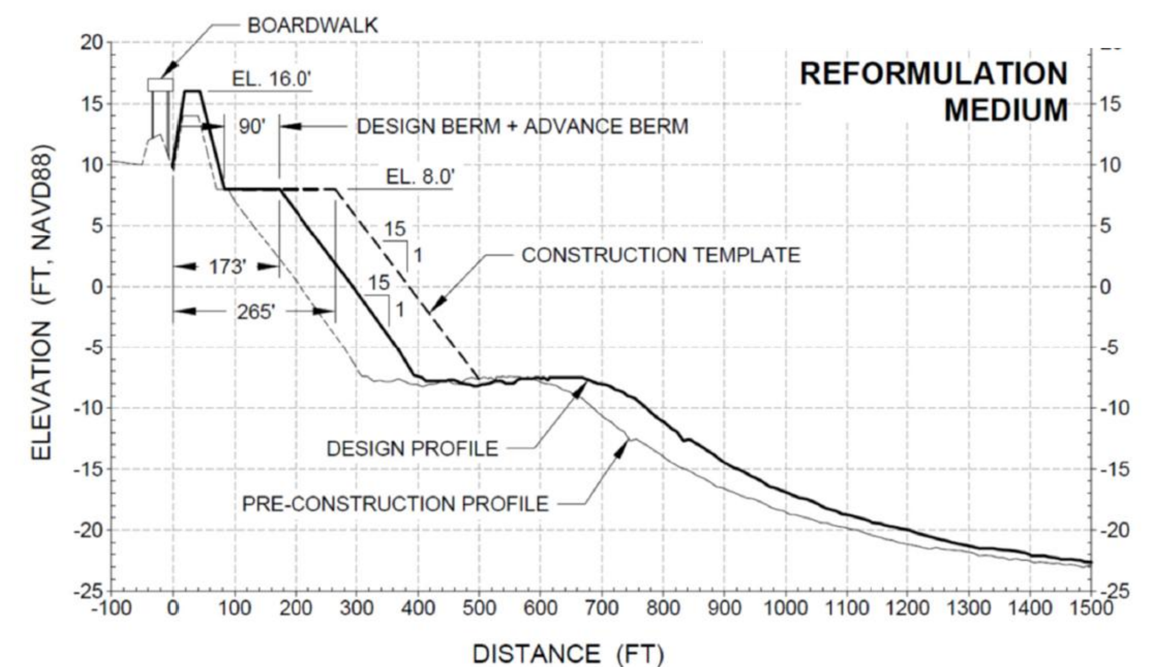
Typical profile of beach berm and dune being considered for Alternatives 1, 2 and 3
