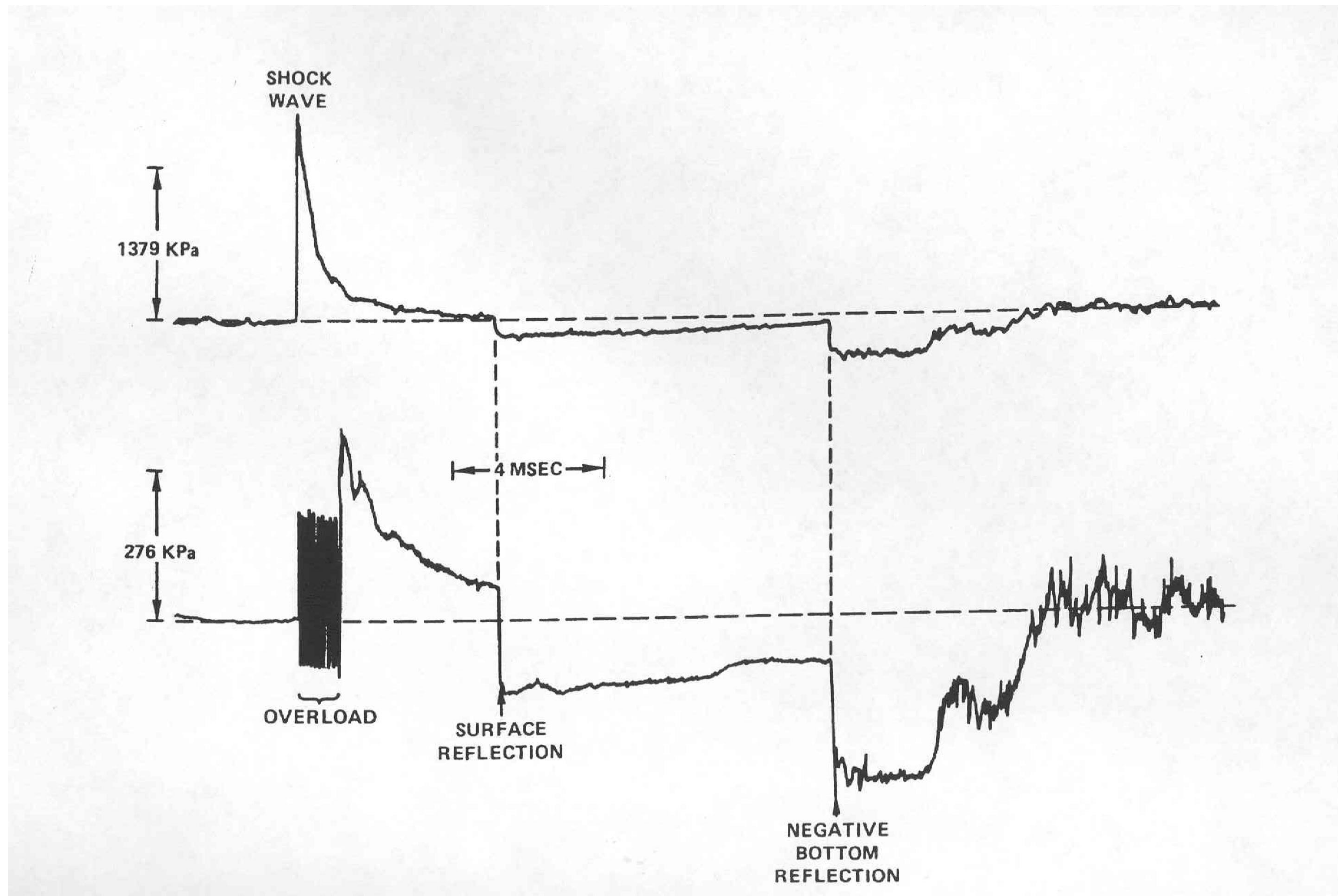
Sample record of pressure shock wave. Gain for upper trace set approximately 5 times lower to show peak pressure ( P_m ). Lower trace provides more detail of negative pressure from reflected waves (from Wiley et al. 1981).
