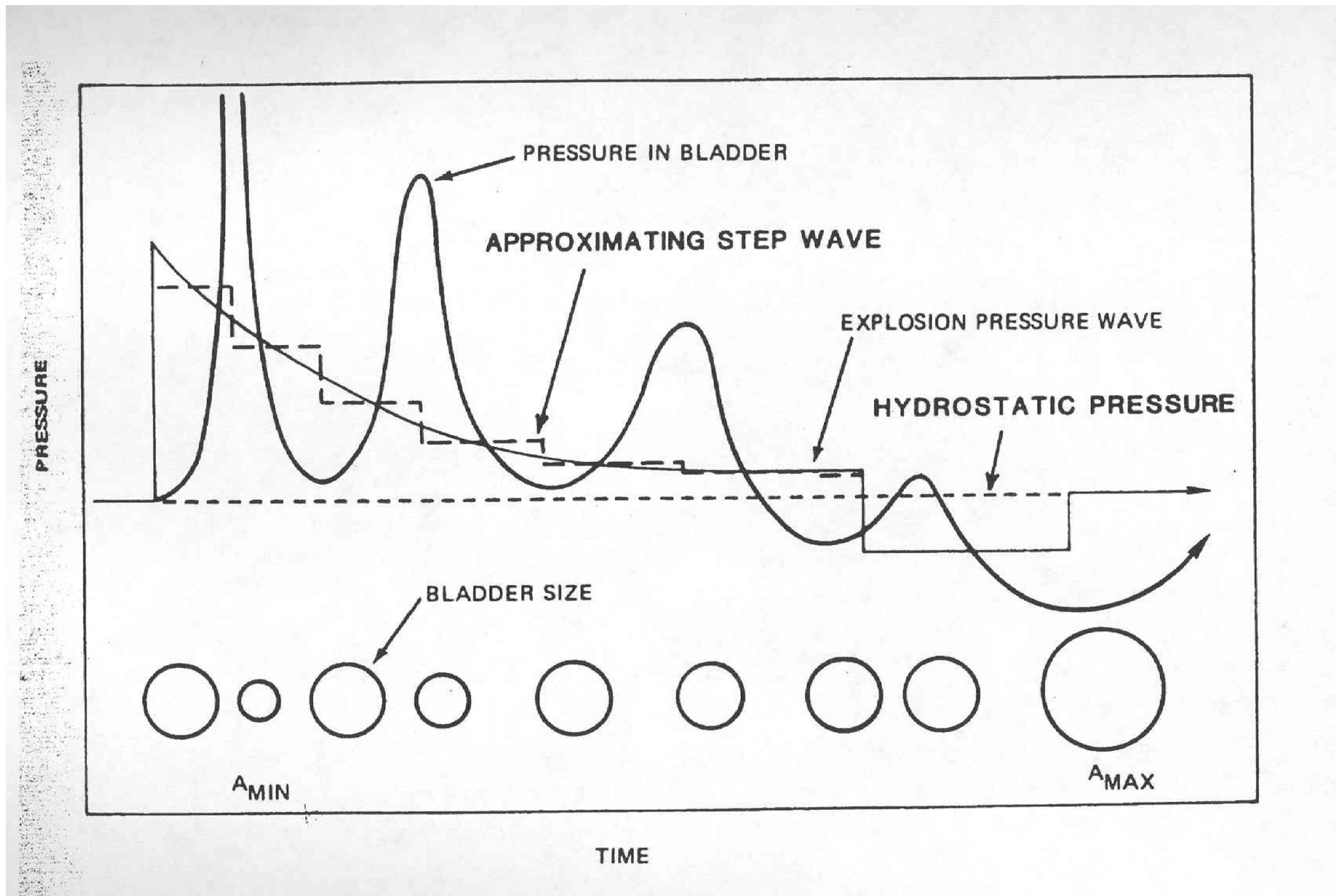
Dynamic model for swimbladder pressure oscillation in response to blast shock pressure wave (from Wiley et al. 1981).
