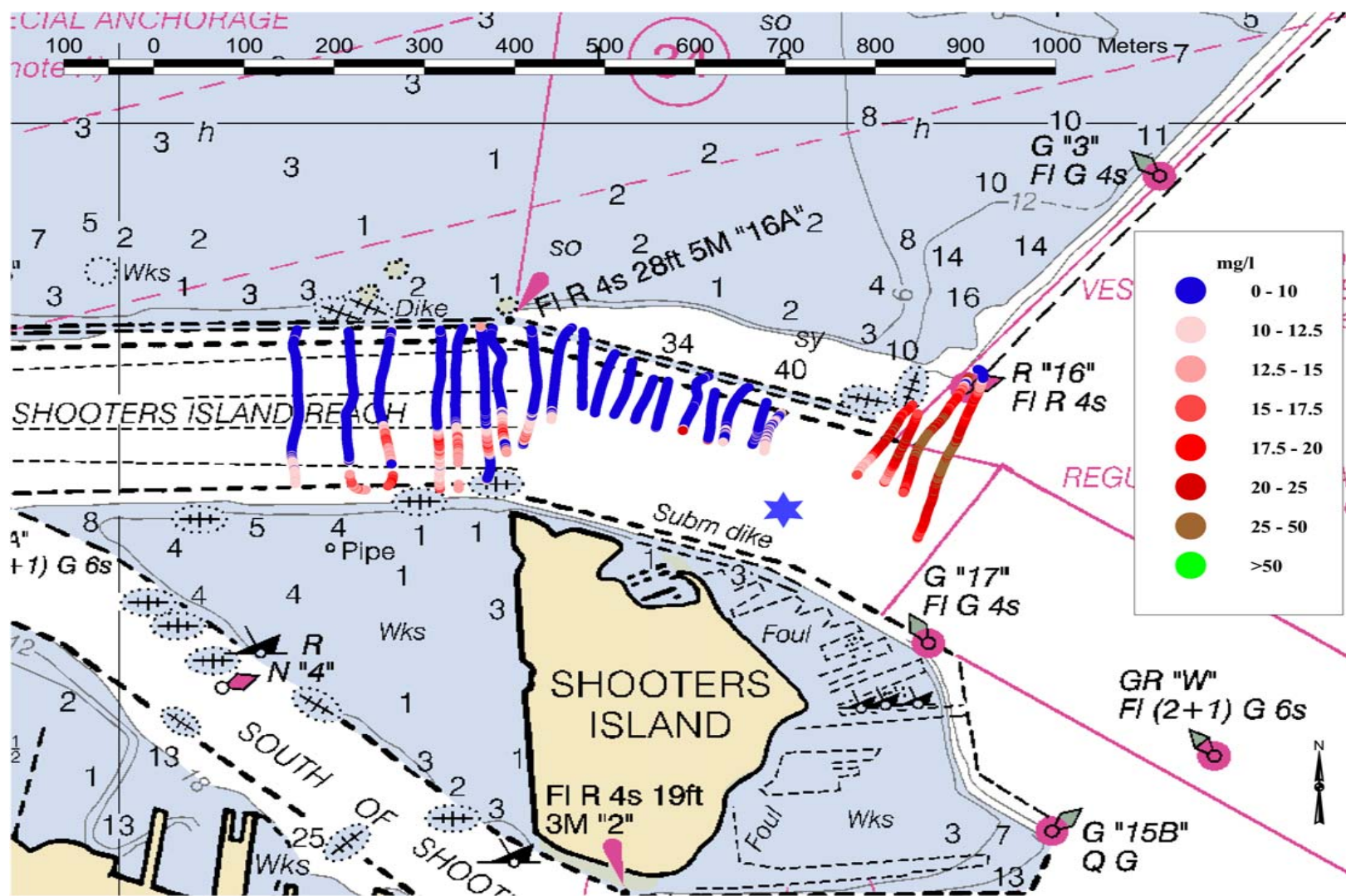
Figure 33. Plan view of detected plume spatial coverage and TSS concentrations at a depth of 12 meters for Survey NJFD, completed during a flooding tide on 20 June 2006.
