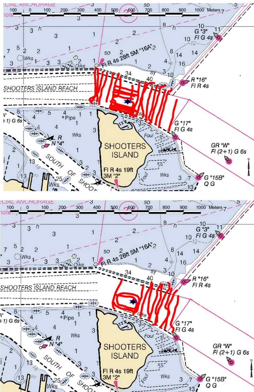
Figure 4. Layout of transects (in red) for ebb tide surveys NJEA (top) and NJEB (bottom). Approximate dredge location denoted by blue star.
