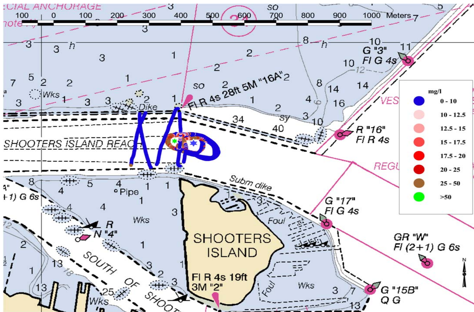
Figure 36. Plan view of detected plume spatial coverage and TSS concentrations at a depth of 2 meters for Survey NJAB, completed during a flooding tide on 22 June 2006. Note: Initial dredge location indicated by a green star, and final position indicated by a blue star, as in following figures.
