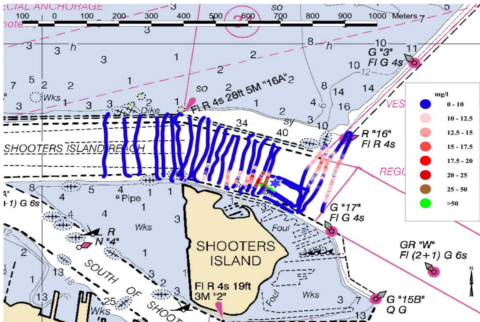
Figure 31. Plan view of detected plume spatial coverage and TSS concentrations at a depth of 8 meters for Survey NJFD, completed during a flooding tide on 20 June 2006.
