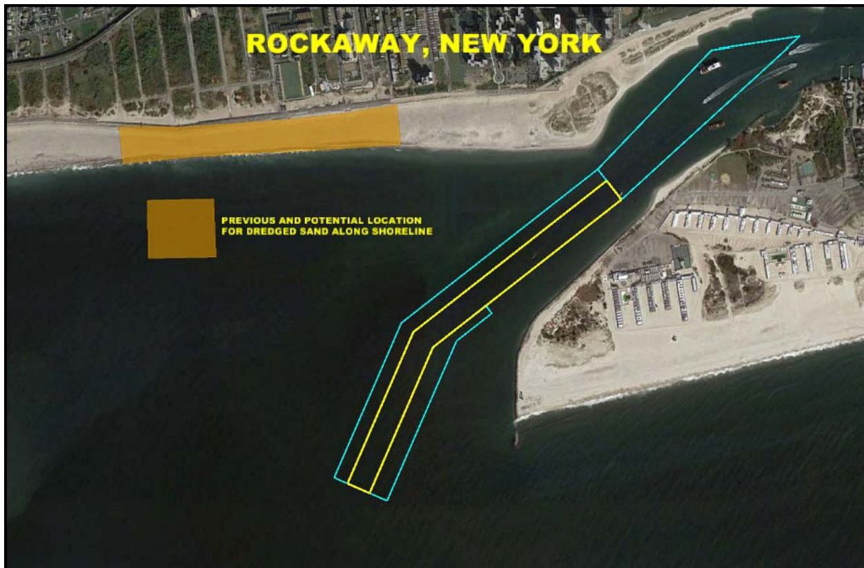
Image 2: Previous and potential East Rockaway Inlet placement location along Rockaway Beach, NY (Google Earth Image Date: October 2014)
